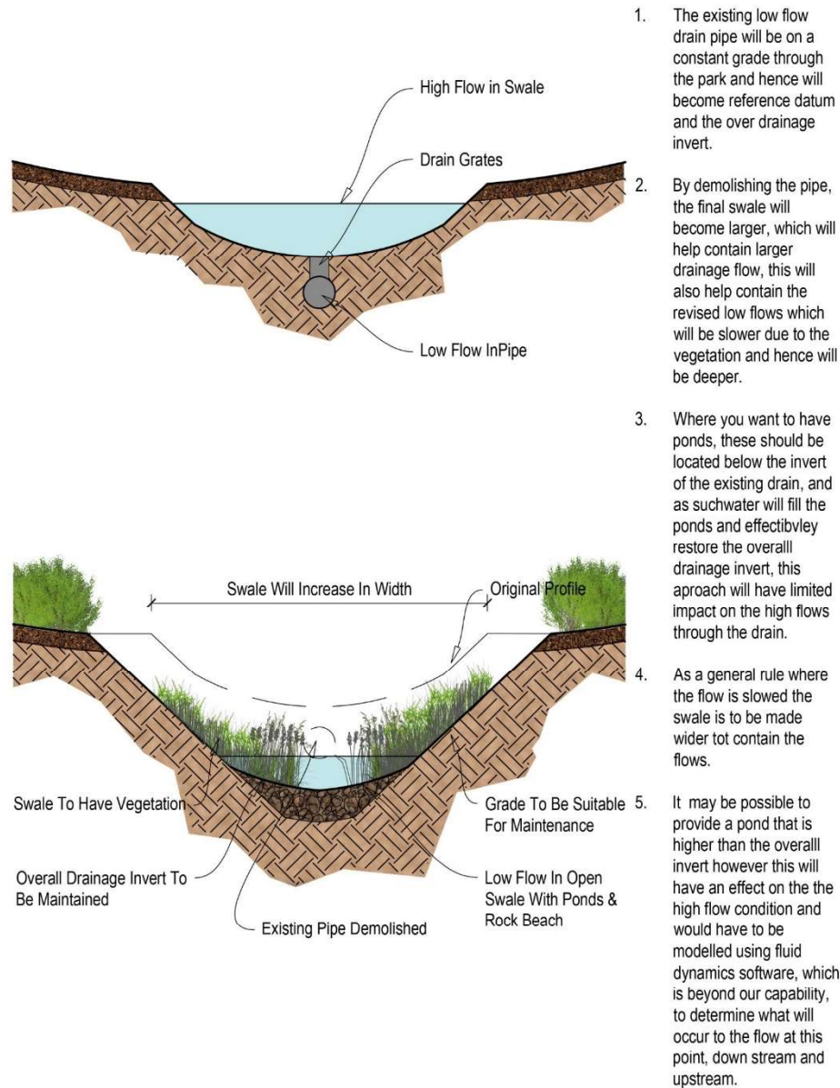
Figure 3: Exposed Low Flow Drainage
